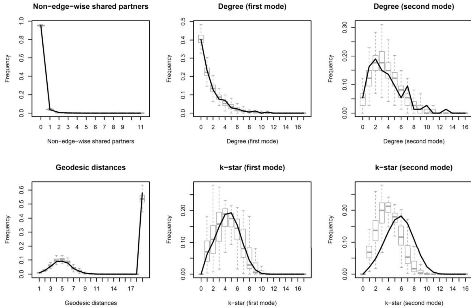
Figure 2. Endogenous Goodness-of-Fit Assessment for Model 1
